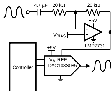
Figure 40. Programmable Attenuator
