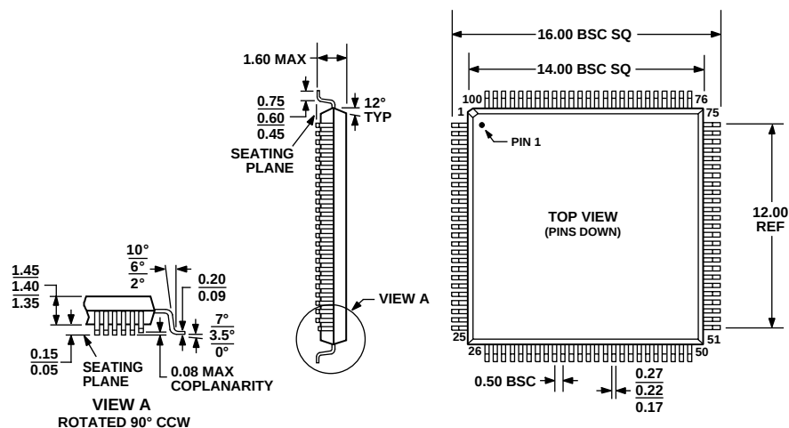
Figure 45. 100-Lead Low Profile Quad Flat Package [LQFP] (ST-100)
