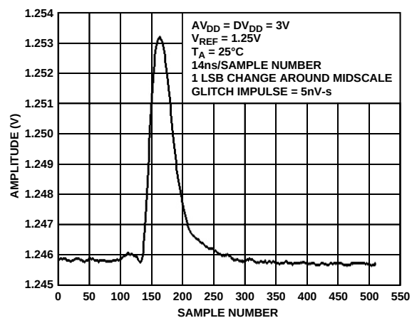
Figure 13. AD5381-3 Glitch Impulse
