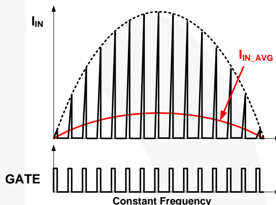
Figure 6. Input Current and Switching
