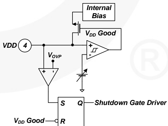
Figure 11. Internal OVP Block
