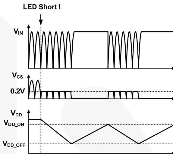
Figure 10. Waveforms in Short-LED Condition
