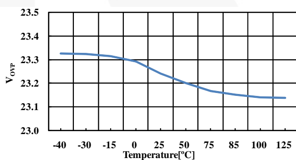
Figure 16. V OVP vs. Temperature
