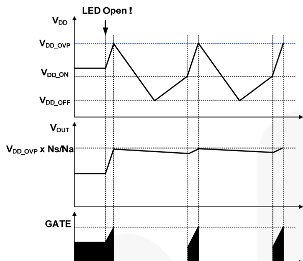
Figure 12. Waveforms in Open-LED Condition
