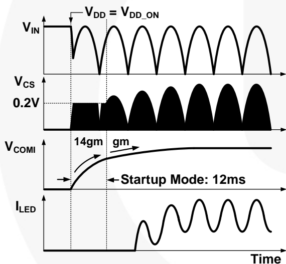
Figure 5. Startup Sequence
