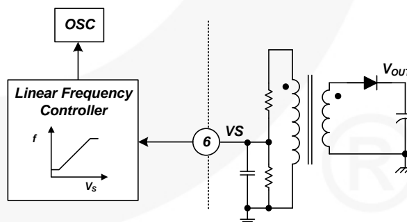
Figure 7. Linear Frequency Control
