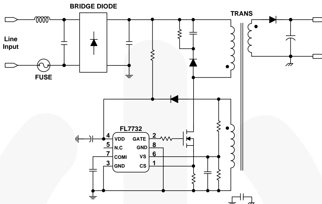
Figure 1. Typical Application
