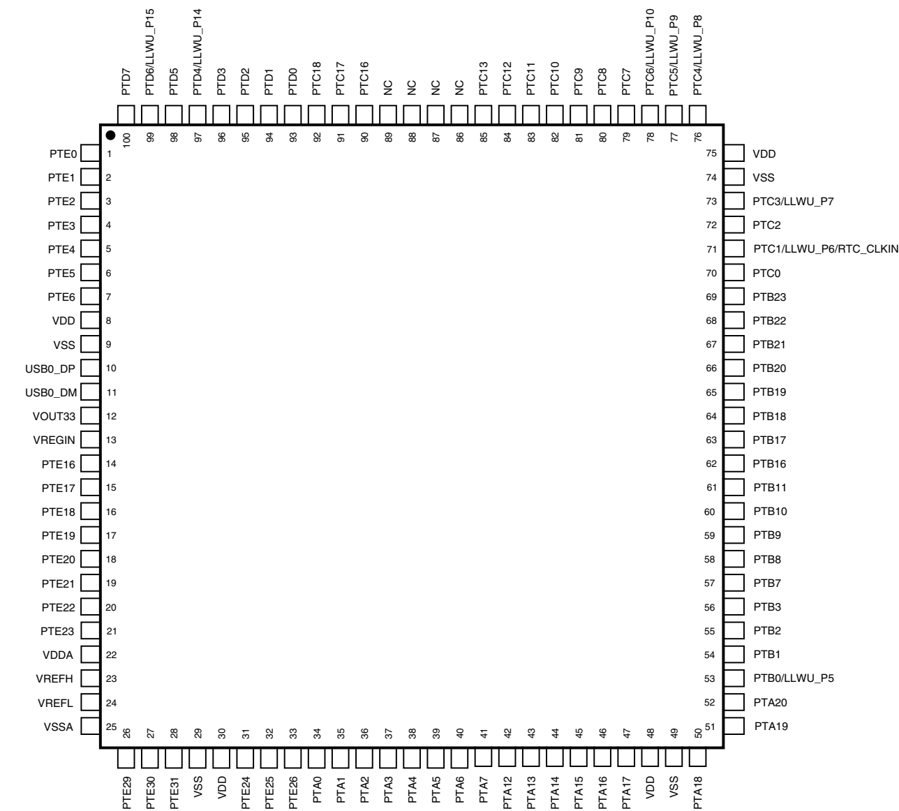
Figure 23. KL26 100-pin LQFP pinout diagram
