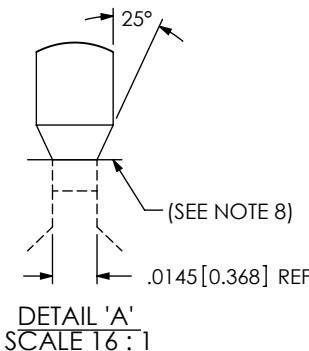
FIG 1 SSQ-1XX-XX-X SHOWN
