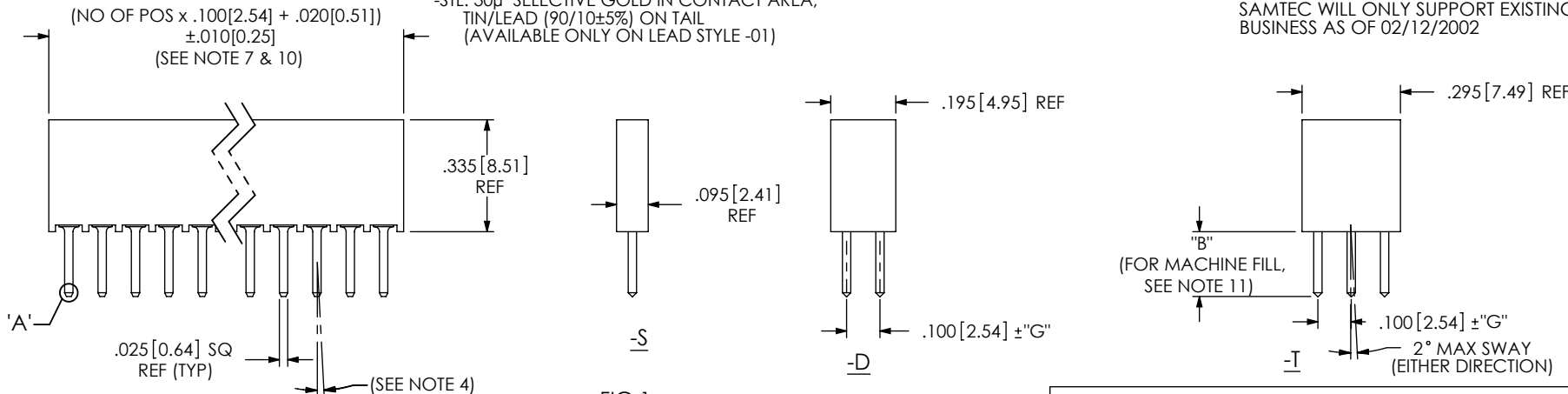
FIG 1 SSQ-1XX-XX-X SHOWN
