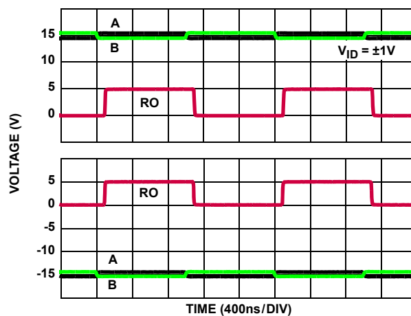
FIGURE 24. RECEIVER PERFORMANCE WITH \pm 15V CMV (ISL32475E)
