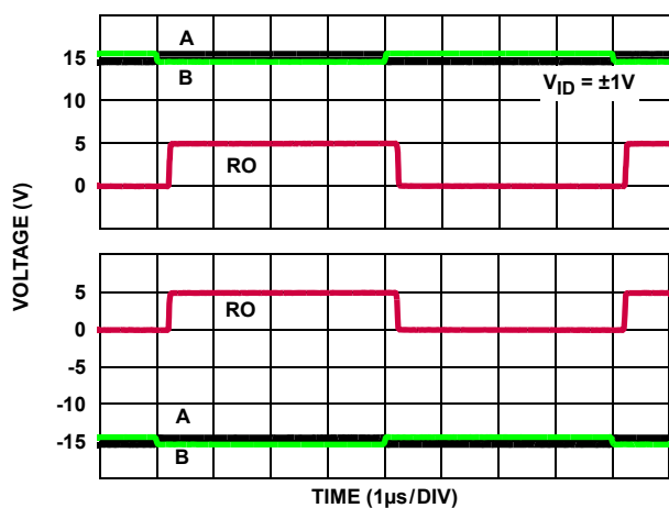
FIGURE 23. RECEIVER PERFORMANCE WITH \pm 15V CMV (ISL32470E, ISL32472E)
