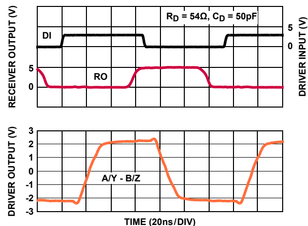
FIGURE 28. DRIVER AND RECEIVER WAVEFORMS (ISL32478E)
