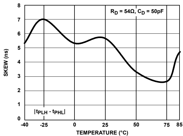
FIGURE 18. DRIVER DIFFERENTIAL SKEW vs TEMPERATURE (ISL32470E, ISL32472E)
