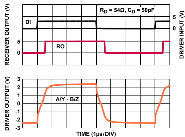
FIGURE 26. DRIVER AND RECEIVER WAVEFORMS (ISL32470E, ISL32472E)
