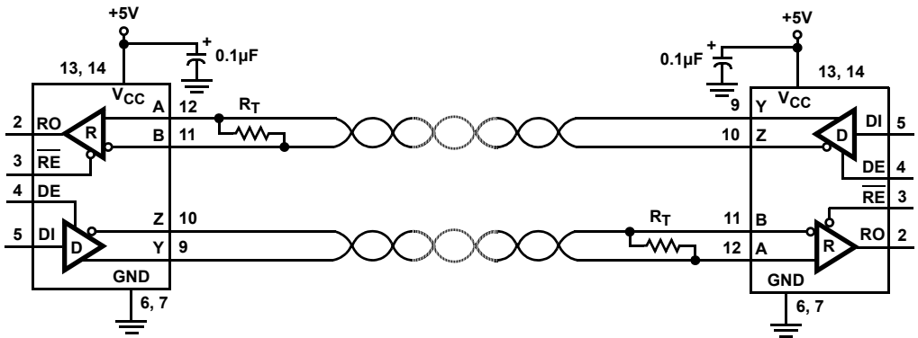
FIGURE 3. ISL32470E FULL DUPLEX EXAMPLE
