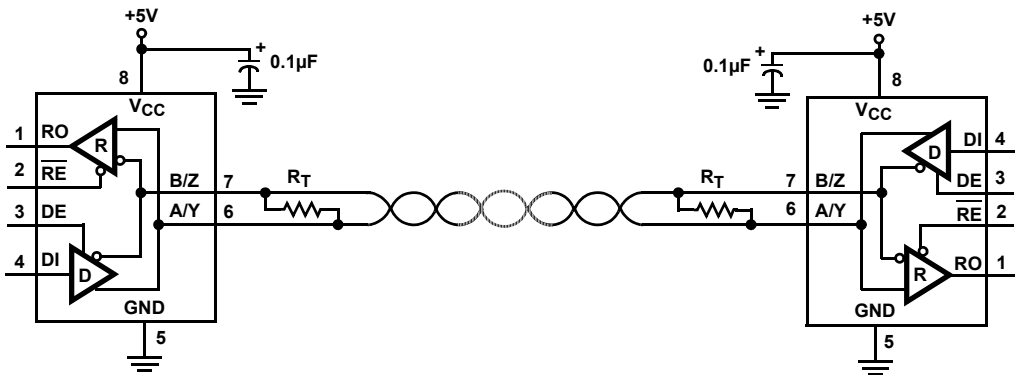
FIGURE 4. ISL32472E, ISL32475E, ISL32478E HALF DUPLEX EXAMPLE
