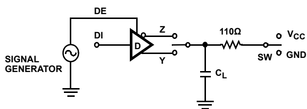
FIGURE 6. DRIVER PROPAGATION DELAY AND DIFFERENTIAL TRANSITION TIMES
