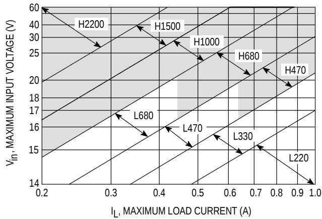
Figure 19. LM2575-12
