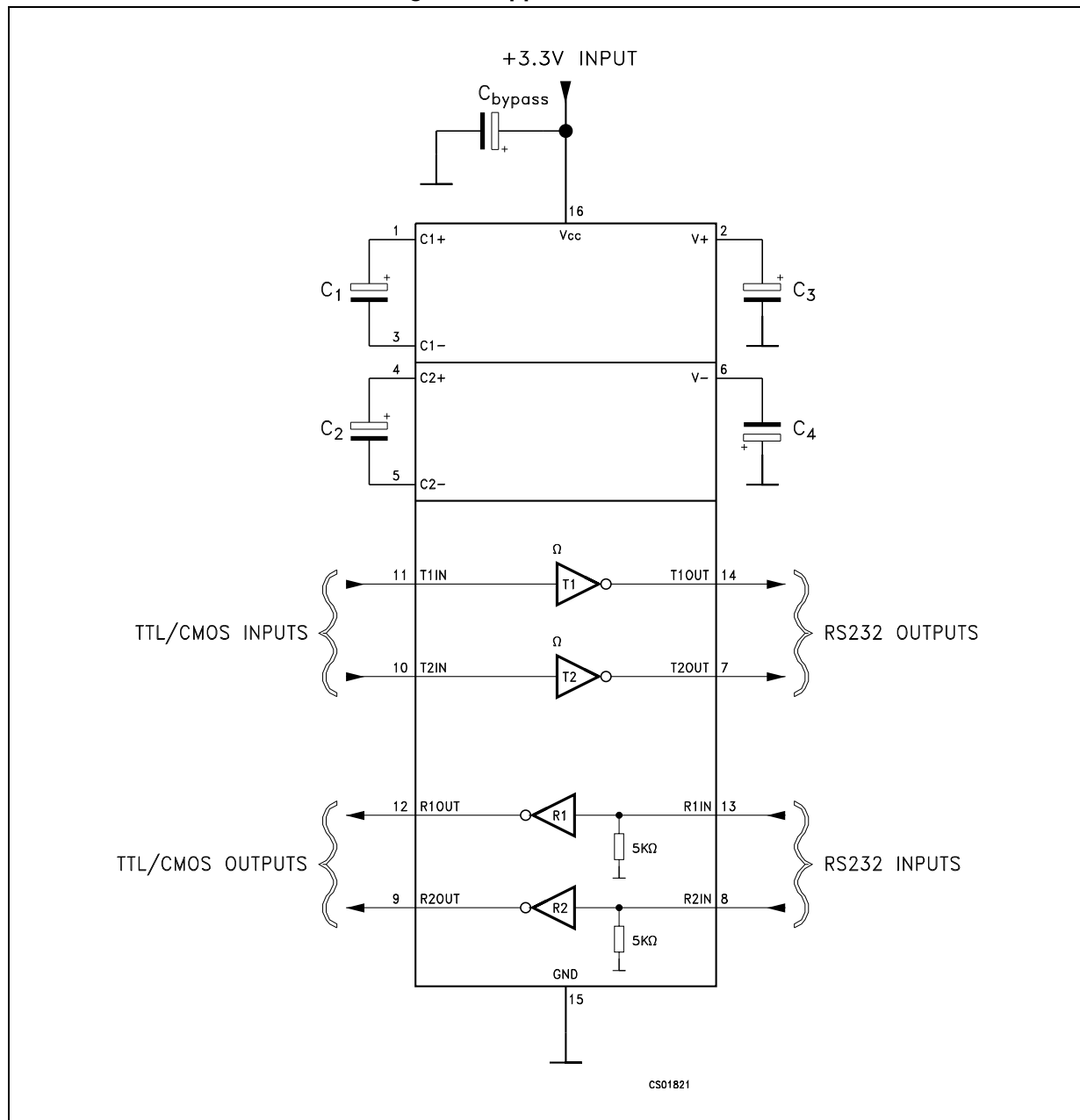
Figure 3. Application circuits
