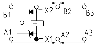
TERMINAL VIEW
