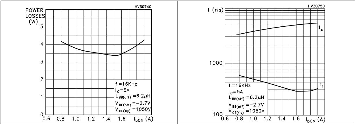
Figure 10. Power losses
