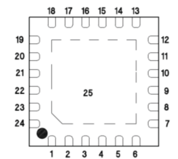
Figure 5 AEAT-8800-Q24: Pins Assignment and Description
