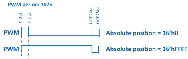
Figure 8 PWM Signals (Period = 1025/2049/4097/8193 \mu\text{s} )
