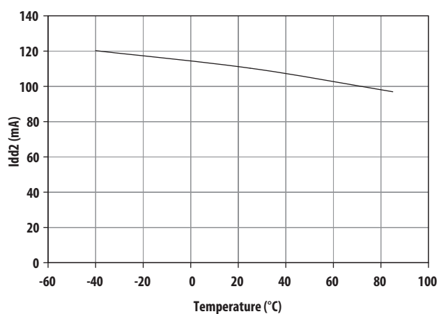
Figure 8. Idd2 vs. Temperature
