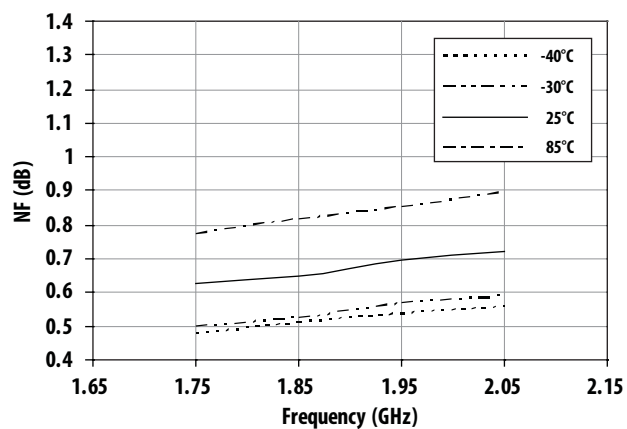
Figure 11. NF vs. Frequency and Temperature
