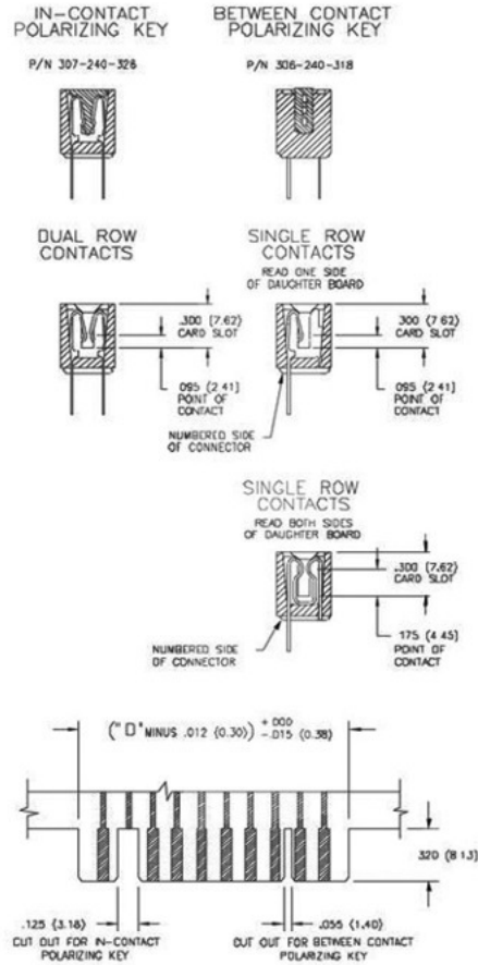
RECOMMENDED DAUGHTER BOARD
