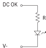
(b) LED
