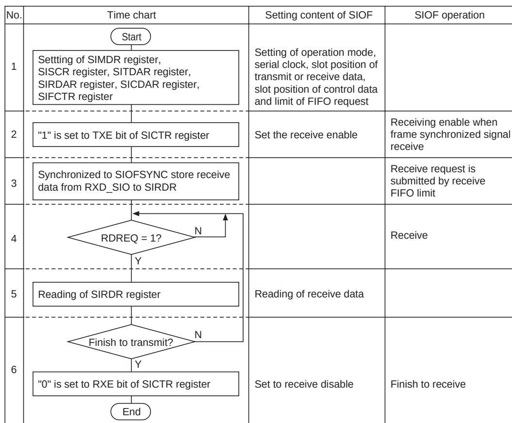
Figure 20.12 Example of Receive Operation in Slave
