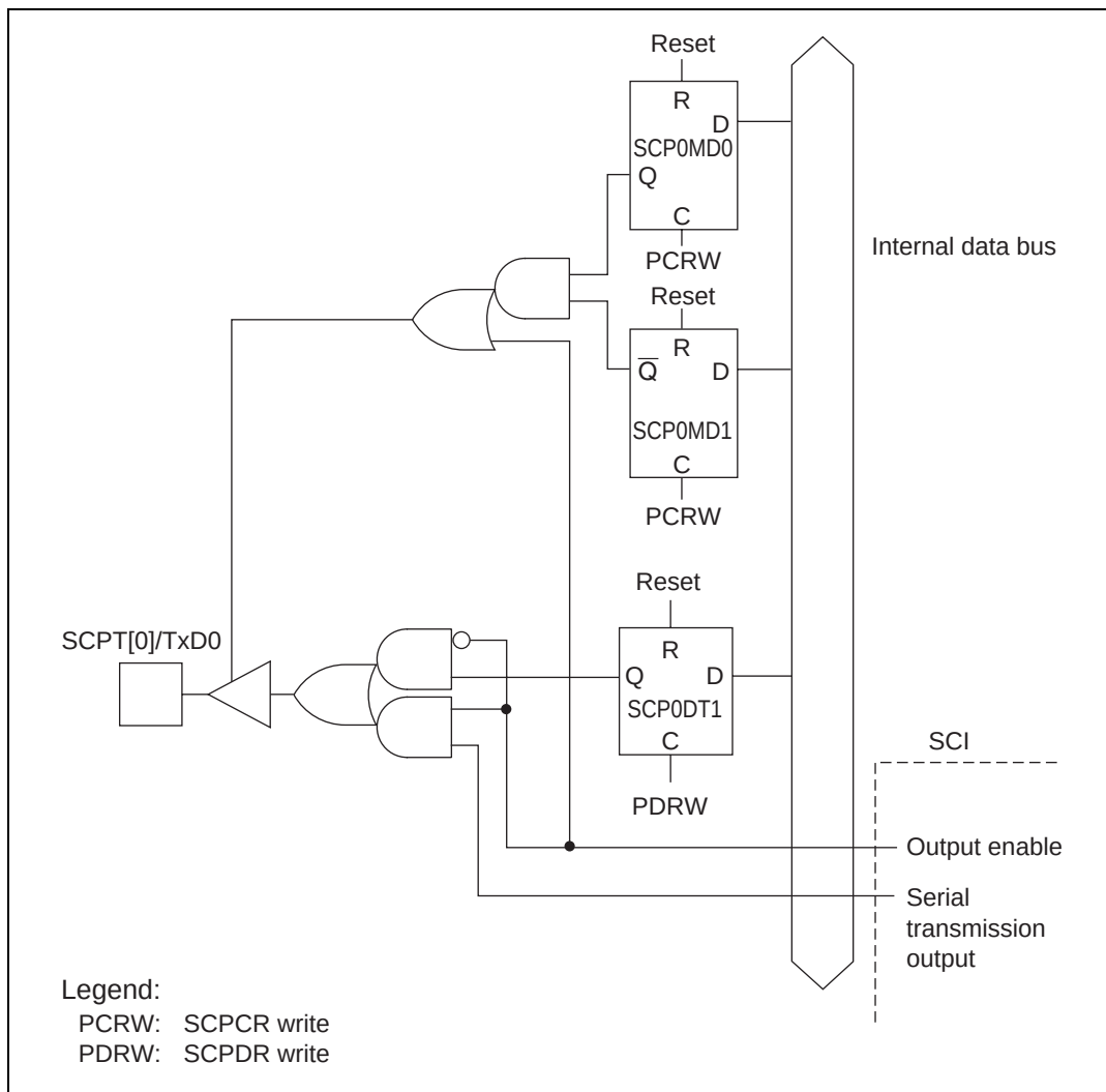
Figure 17.3 SCPT[0]/TxD0 Pin
