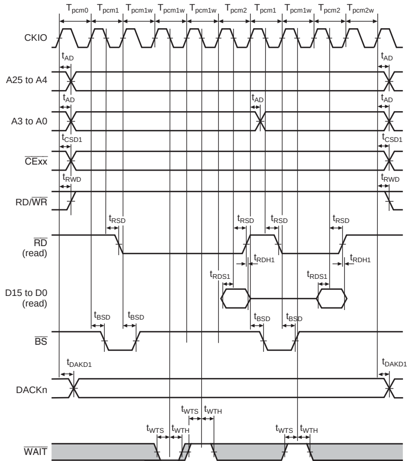
Figure 32.37 PCMCIA Memory Bus Cycle (Burst Read, TED = 1, TEH = 1, Two Waits, Burst Pitch = 3, WAITSEL = 1)
