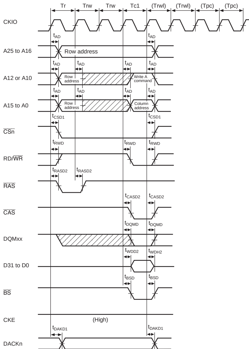
Figure 32.28 Synchronous DRAM Write Bus Cycle (RCD = 2, TPC = 1, TRWL = 1)
