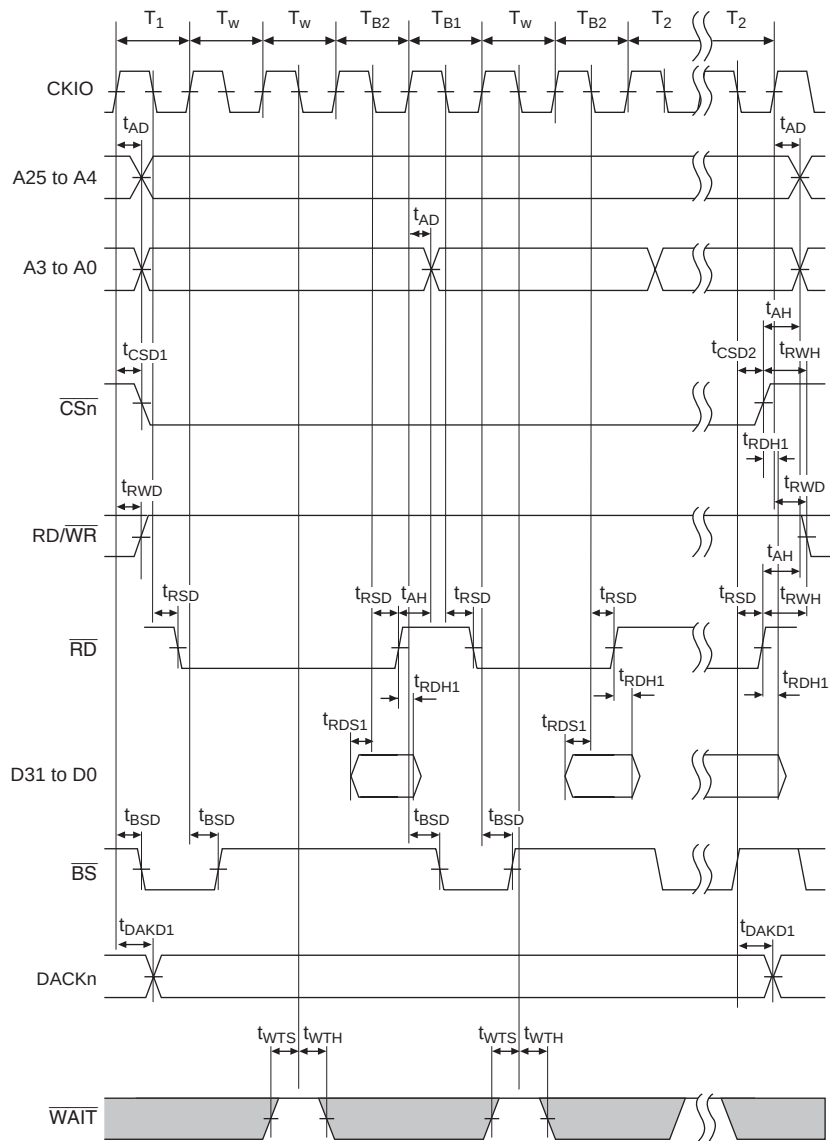
Figure 32.21 Burst ROM Bus Cycle (Two Waits)
