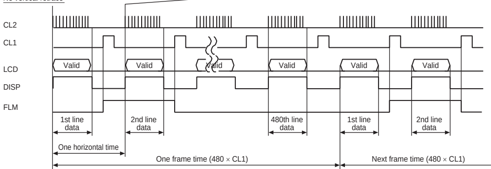
Figure 25.21 Clock and LCD Data Signal Example
