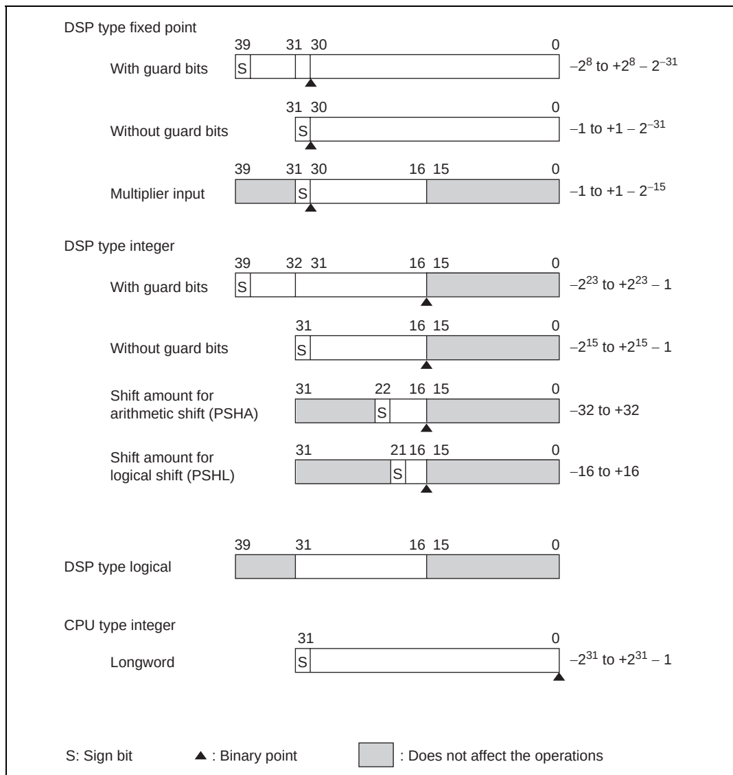
Figure 2.10 Data Format
