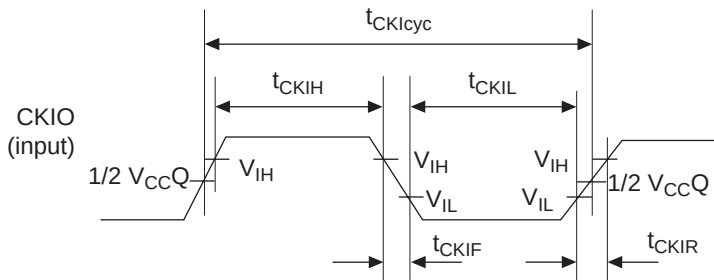
Figure 32.4 CKIO Clock Input Timing
