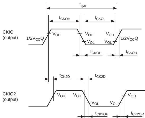
Figure 32.5 CKIO Clock Output Timing
