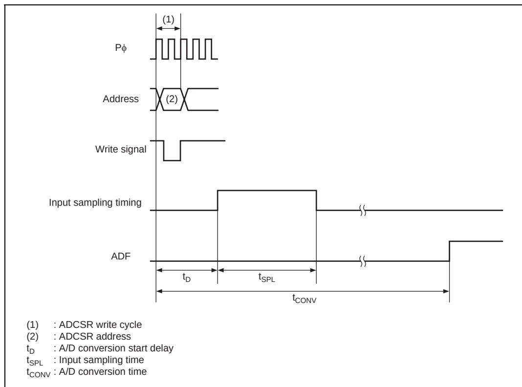
Figure 28.6 A/D Conversion Timing
