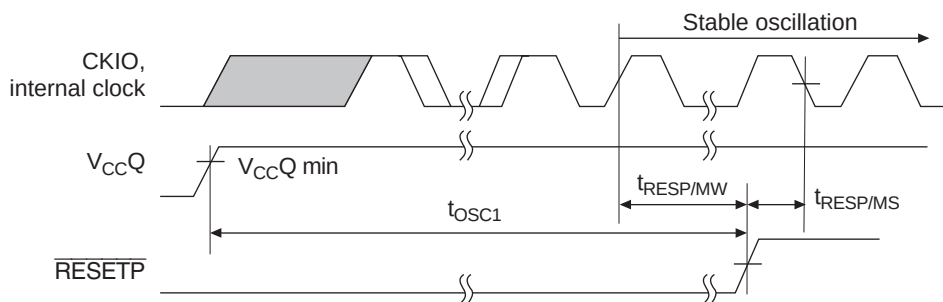
Figure 32.5 CKIO Clock Output Timing
