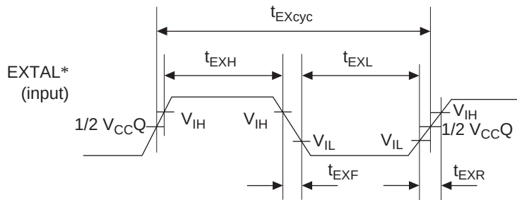
Figure 32.3 EXTAL Clock Input Timing
