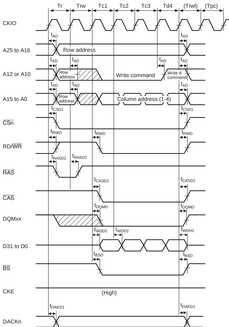
Figure 32.30 Synchronous DRAM Write Bus Cycle (Burst Mode (Single Write × 4), RCD = 1, TPC = 0, TRWL = 0)
