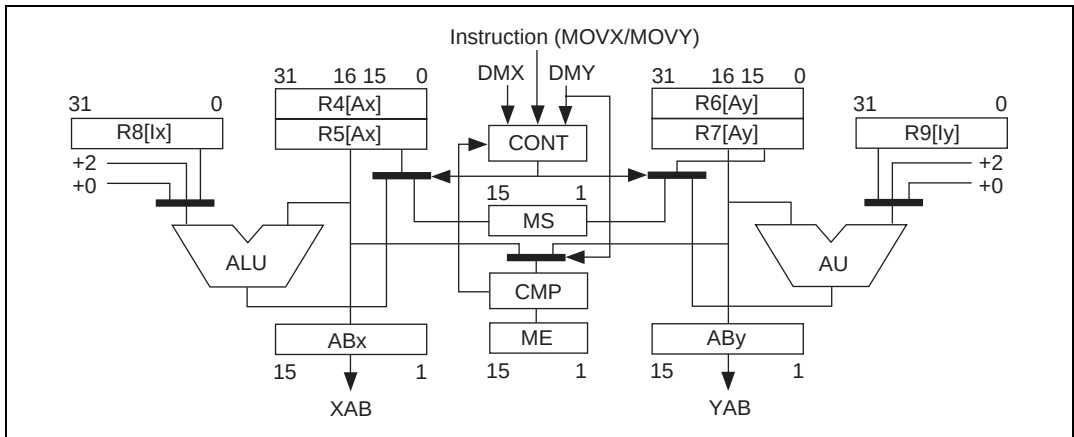
Figure 2.14 Modulo Addressing
