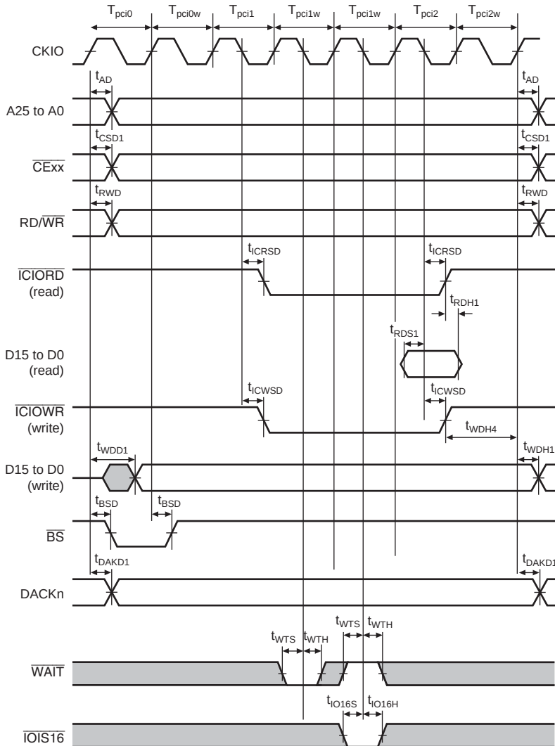
Figure 32.39 PCMCIA I/O Bus Cycle (TED = 2, TEH = 1, One Wait, External Wait, WAITSEL = 1)
