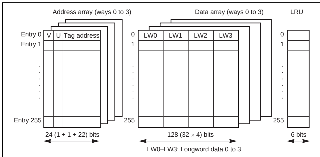
Figure 5.1 Cache Structure
