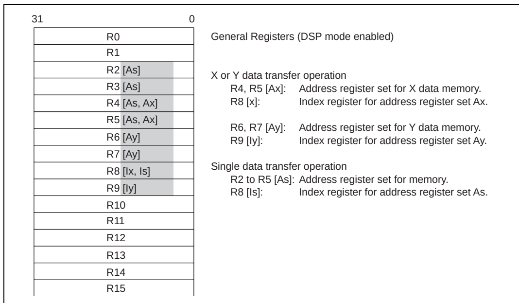
Figure 2.4 General Purpose Register (DSP Mode)
