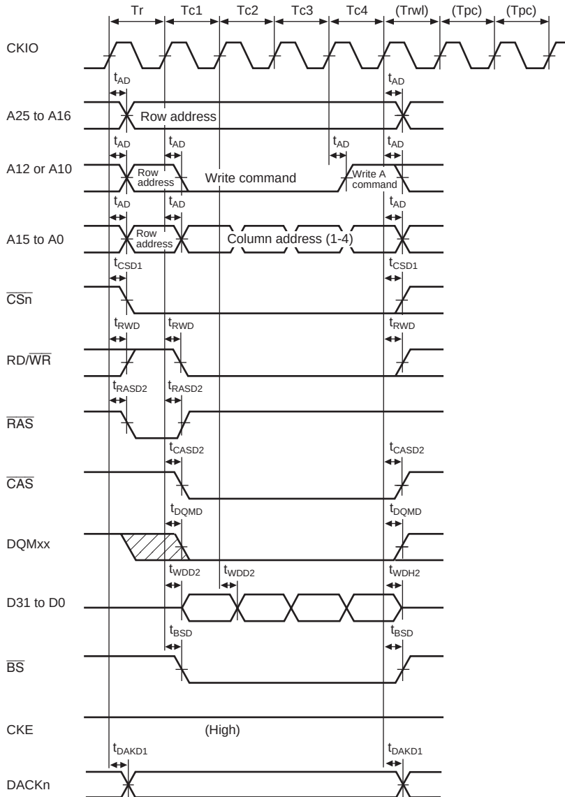
Figure 32.29 Synchronous DRAM Write Bus Cycle (Burst Mode (Single Write × 4), RCD = 0, TPC = 1, TRWL = 0)
