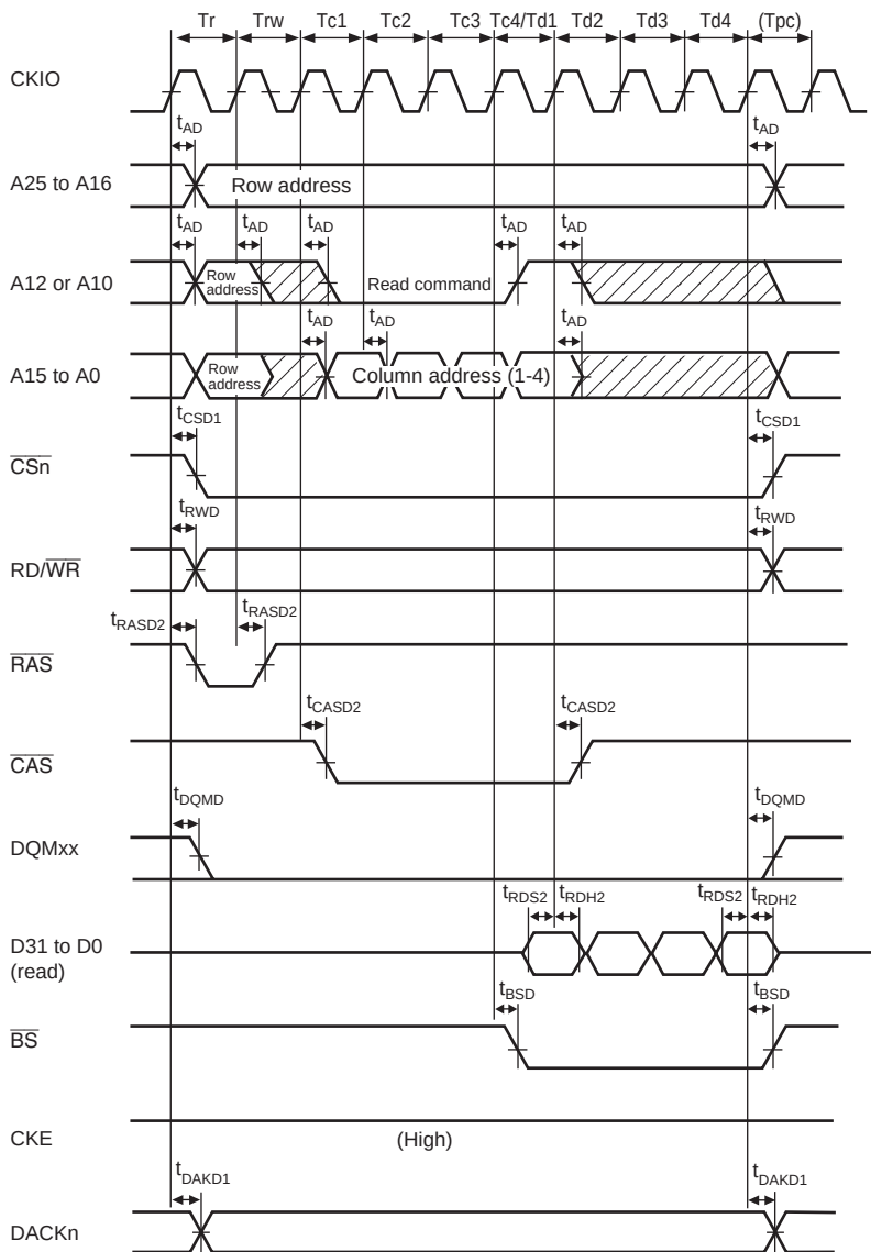
Figure 32.26 Synchronous DRAM Read Bus Cycle (Burst Read (Single Read \times 4), RCD = 1, CAS Latency = 3, TPC = 0)
