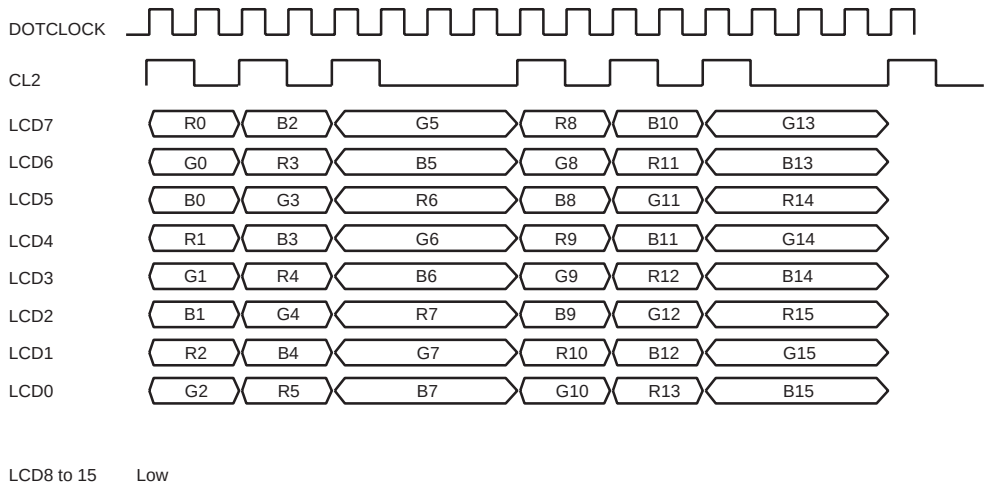
Figure 25.11 Clock and LCD Data Signal Example
