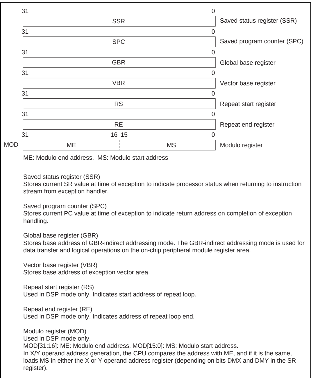
Figure 2.5 Control Registers (2)
