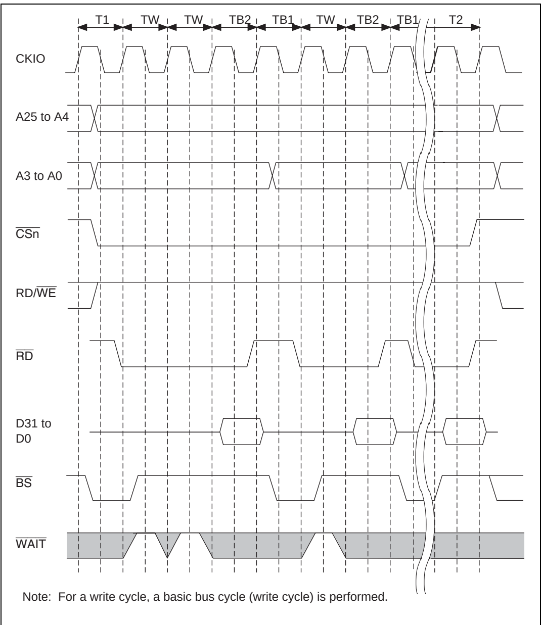
Figure 12.22 Burst ROM Wait Access Timing
