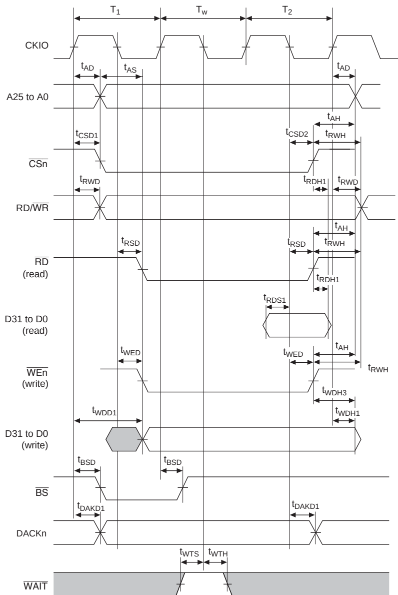
Figure 32.18 Basic Bus Cycle (One Wait)
