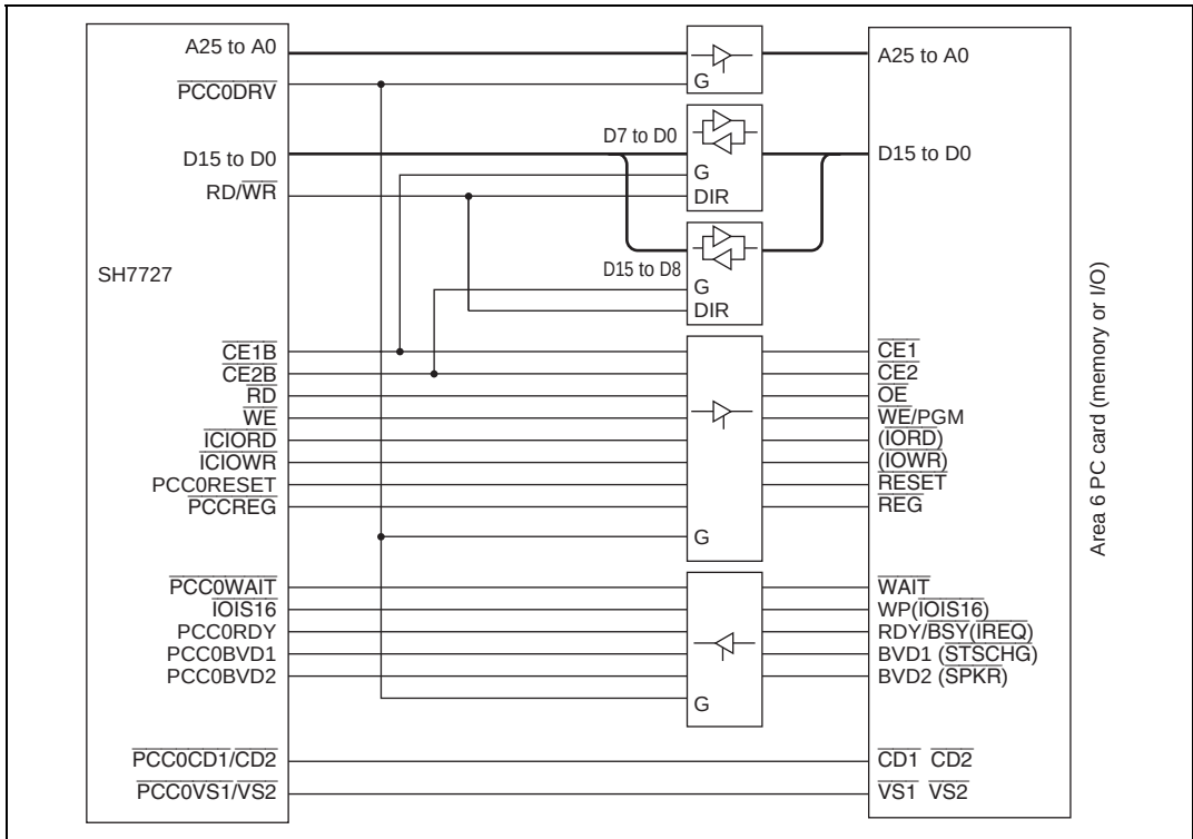
Figure 30.4 SH7727 Interface
