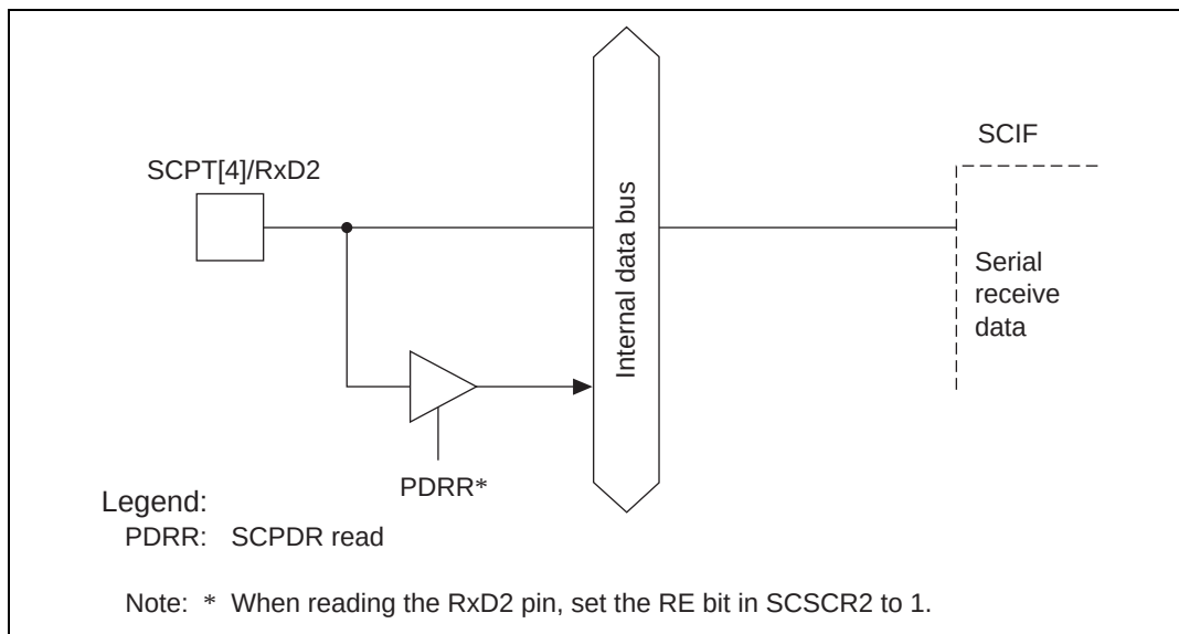
Figure 19.3 SCPT[4]/RxD2 Pin
