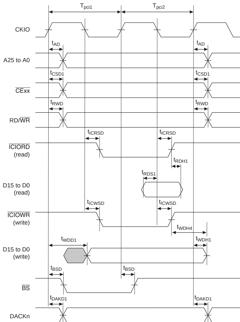
Figure 32.38 PCMCIA I/O Bus Cycle ( TED = 0 , TEH = 0 , No Wait)
