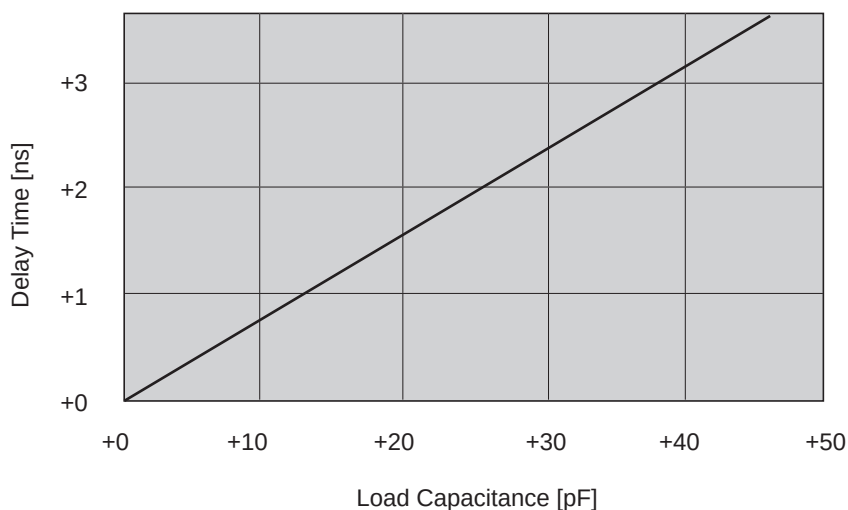
Figure 32.61 Load Capacitance vs. Delay Time
