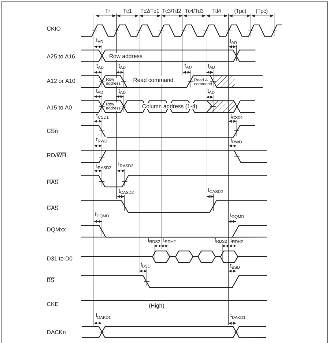
Figure 32.25 Synchronous DRAM Read Bus Cycle (Burst Read (Single Read × 4), RCD = 0, CAS Latency = 1, TPC = 1)
