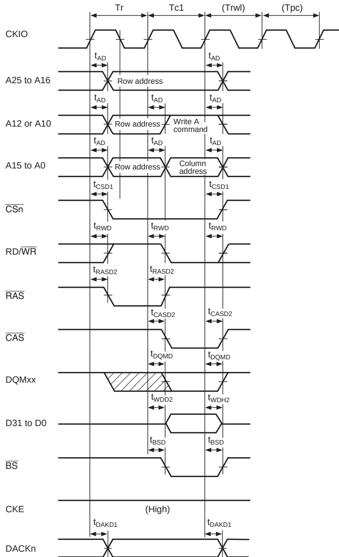
Figure 32.27 Synchronous DRAM Write Bus Cycle ( RCD = 0 , TPC = 0 , TRWL = 0 )
