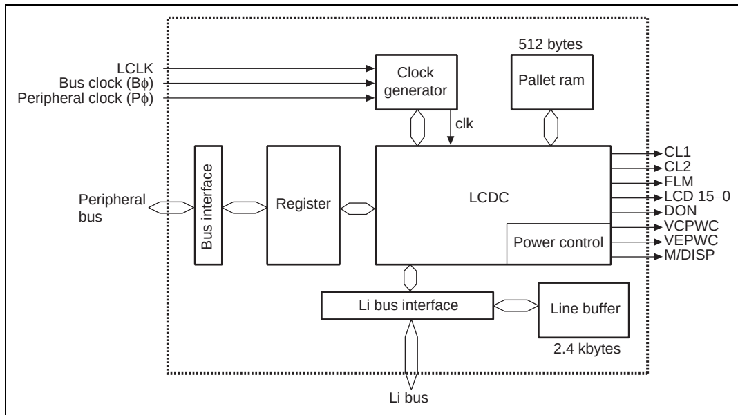
Figure 25.1 Block Diagram
