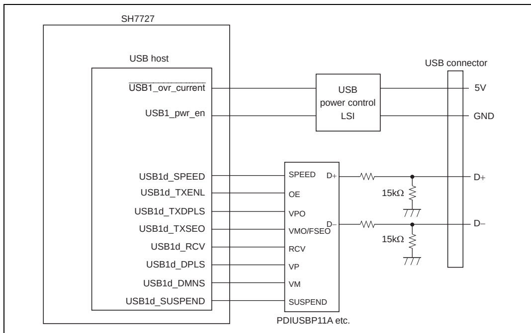
Figure 22.7 Example 2 of Transceiver Connection for USB Host Controller (On-chip transceiver is not used)
