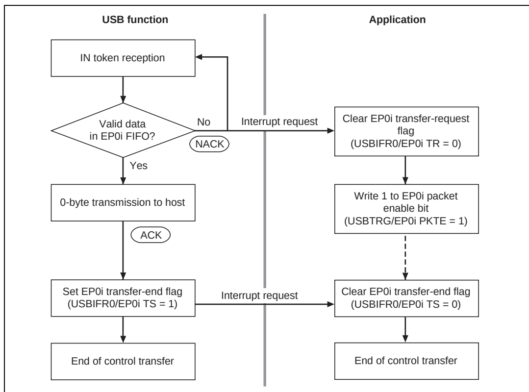
Figure 23.9 Status Stage Operation (Control-Out)
