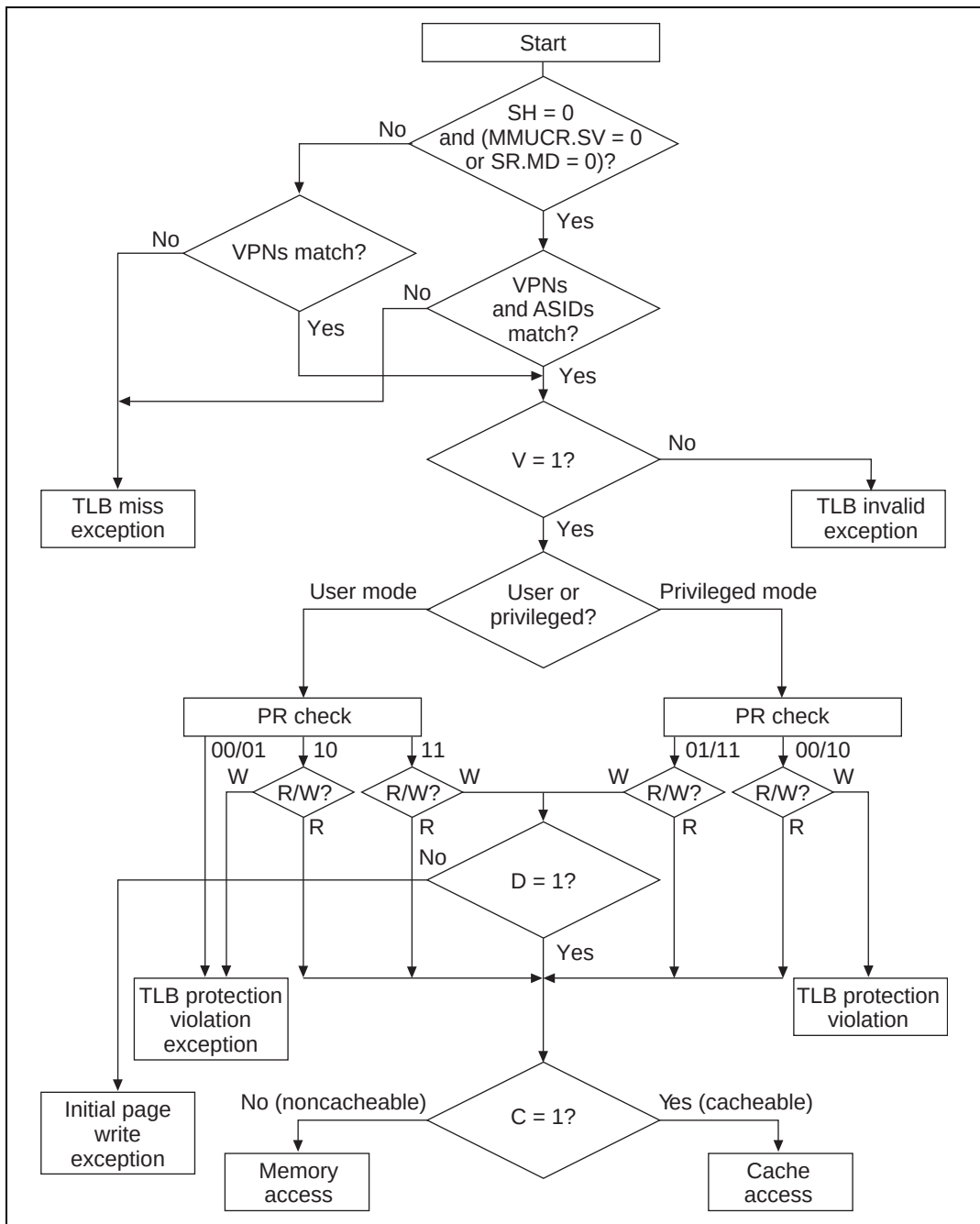
Figure 3.11 MMU Exception Generation Flowchart
