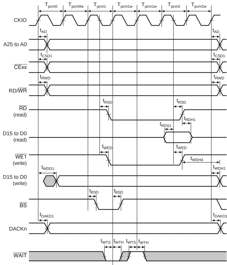
Figure 32.35 PCMCIA Memory Bus Cycle (TED = 2, TEH = 1, One Wait, External Wait, WAITSEL = 1)
