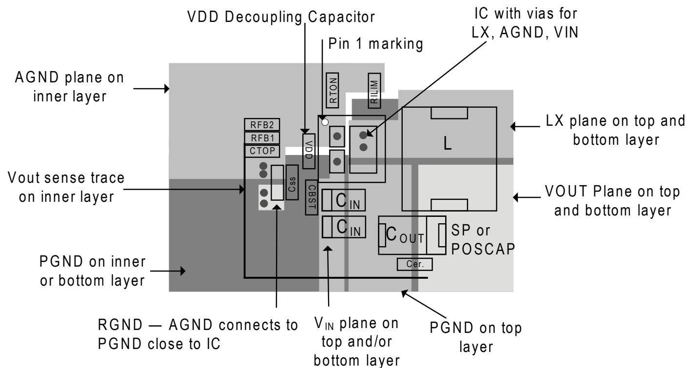
Figure 14 — PCB Layout
