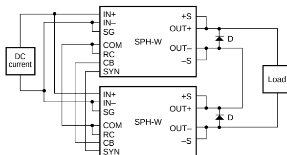
Fig.10 Connection for serial operation
