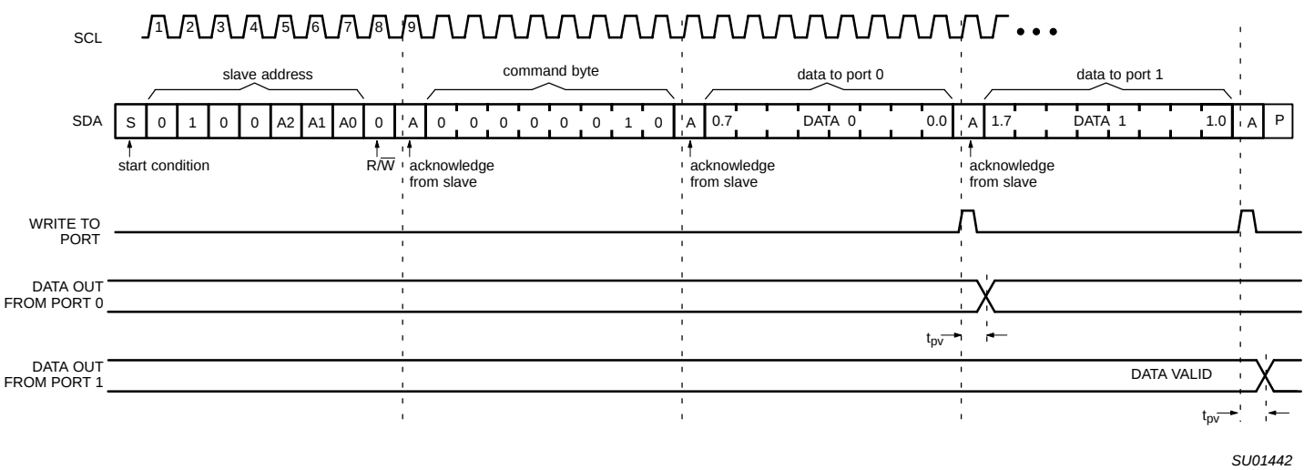
Figure 6. WRITE to output port registers
