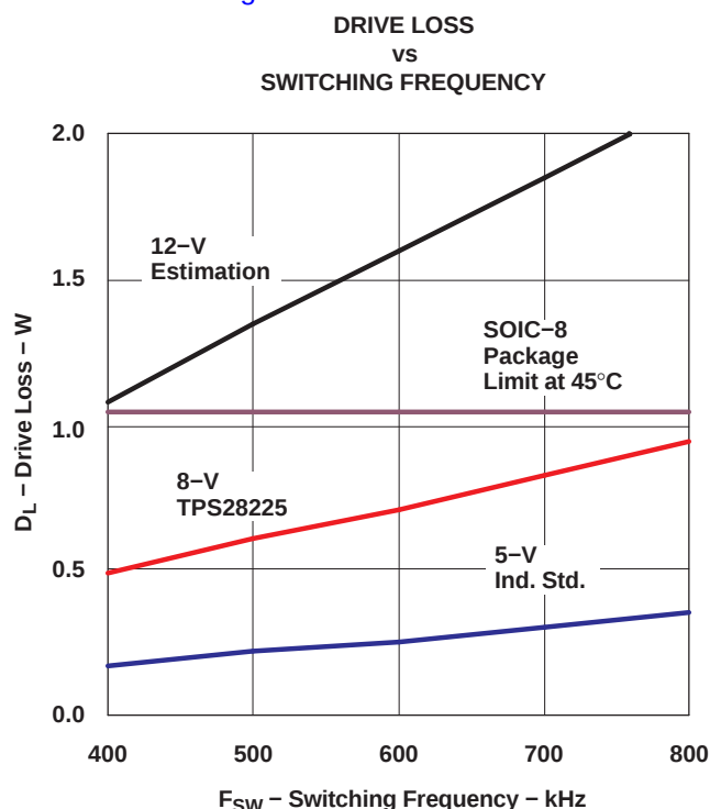
Figure 37. Drive Power as Function of V_{GS} and F_{SW}
