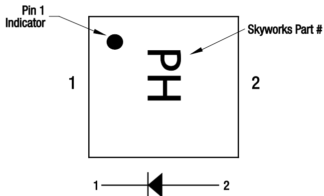
Figure 4. Typical Case Markings (Top View)
