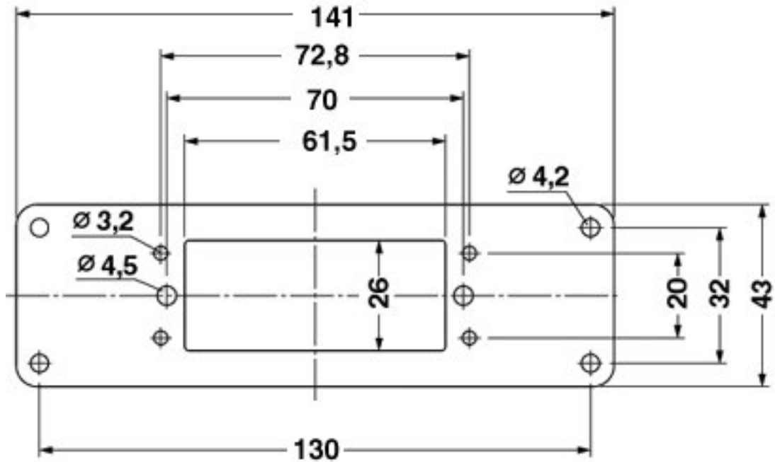
Dimensioned drawing
