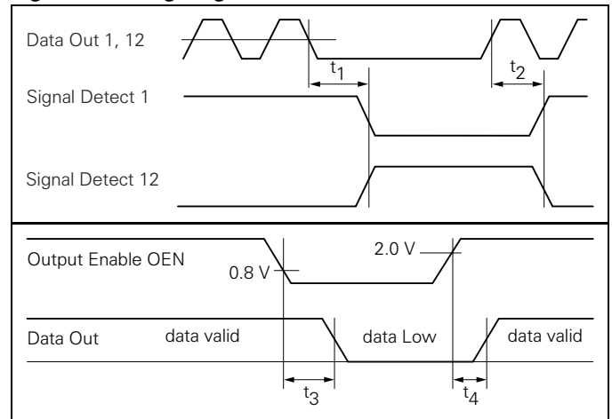
Figure 8. Timing diagrams
