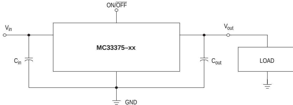
Figure 22. Typical Application Circuit
