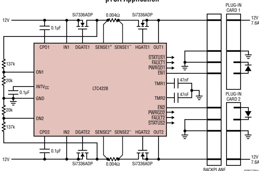
\mu\text{TCA} Application
