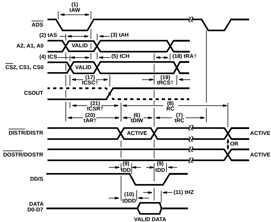
FIGURE 7. READ CYCLE
