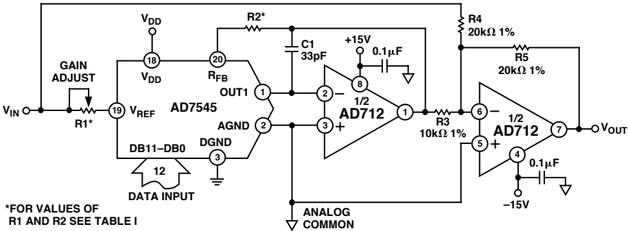
Figure 9. Bipolar Operation
