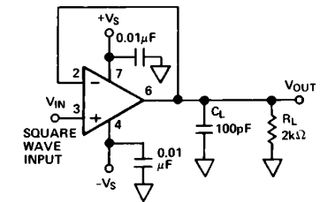
Figure 21c. Unity Gain Follower-AD542/AD547
