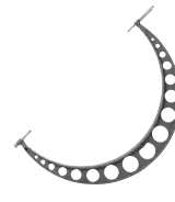
V-Anvil Micrometers SERIES 314, 114
