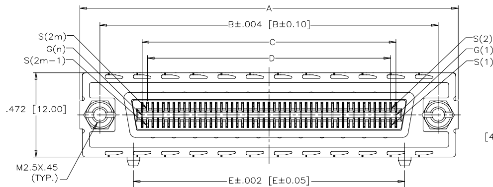
FRONT VIEW U65-EXX-XX2XXX
