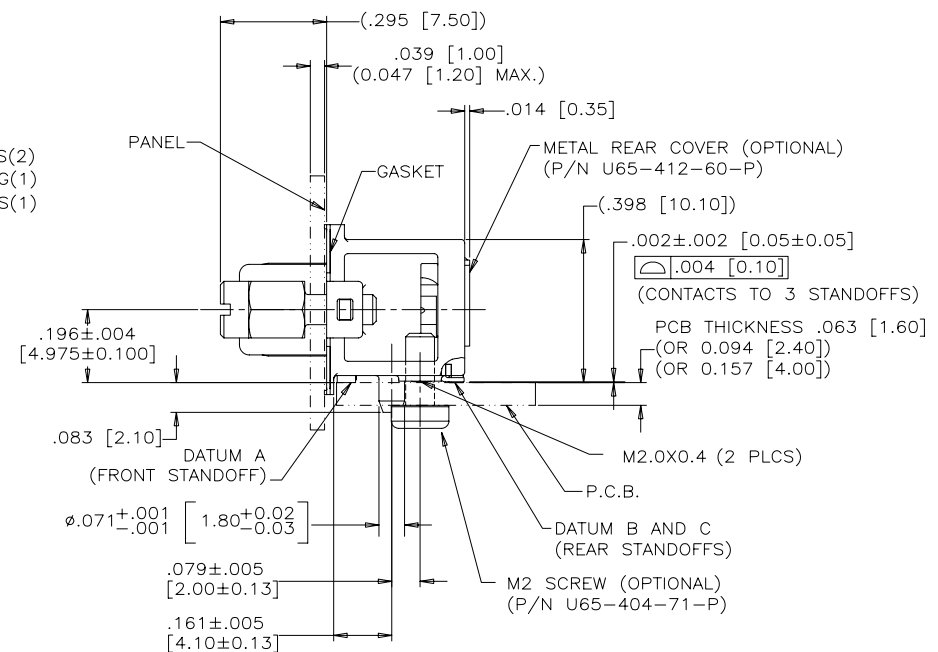
SIDE VIEW U65-EXX-XX2XXX
