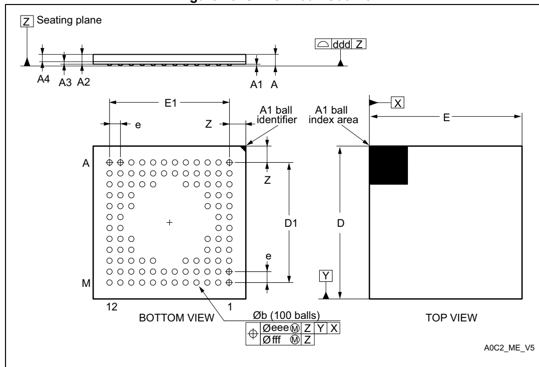
Figure 45. UFBGA100 - Outline
