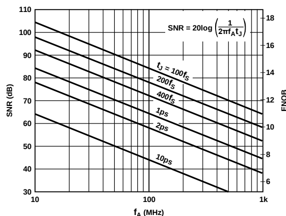
Figure 70. SNR and ENOB vs. Analog Input Frequency
