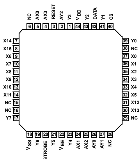
CD22M3494MQ (PLCC) (MITEL LEAD COMPATIBLE) TOP VIEW
