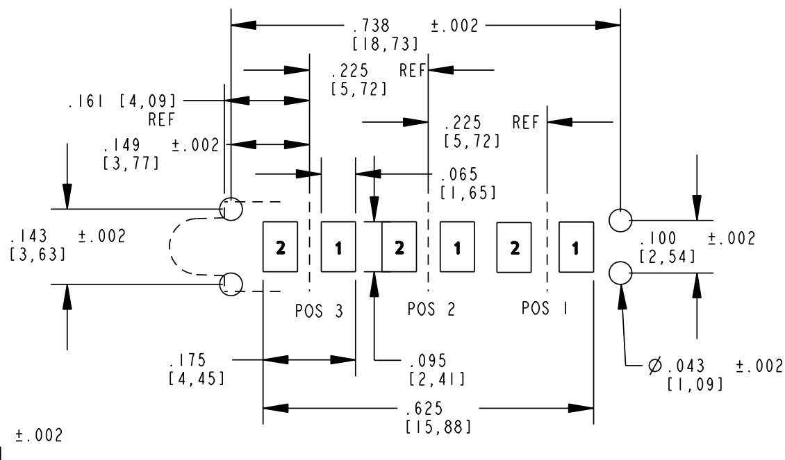
FIG. 1 RECOMMENDED PAD LAYOUT - SINGLE COLOR LEDS
