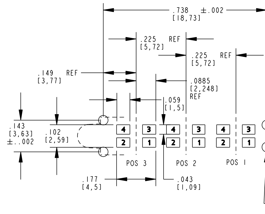
FIG. 2 RECOMMENDED PAD LAYOUT - MULTI-COLOR LEDS
