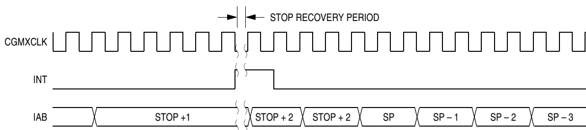
Figure 13-15. Stop Mode Recovery from Interrupt
