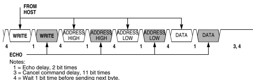
Figure 16-13. Write Transaction
