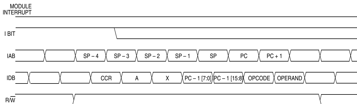
Figure 13-8. Interrupt Recovery
