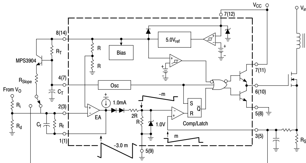
Figure 33. Slope Compensation
