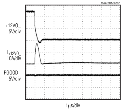
+12VO_ IMMEDIATE SHORT-CIRCUIT RESPONSE
