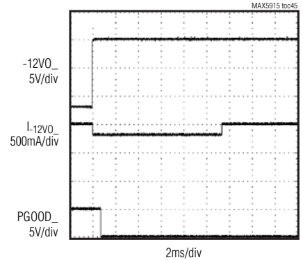
-12VO_ CURRENT FOLDBACK
