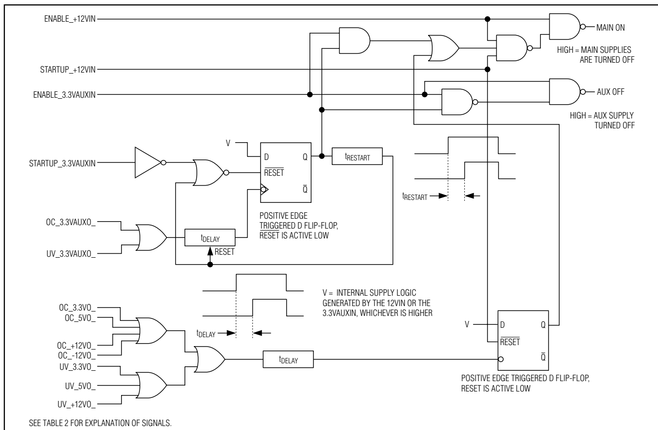
Figure 3. Main and Auxiliary Supply Shutdown Control Logic for MAX5915/MAX5915A
