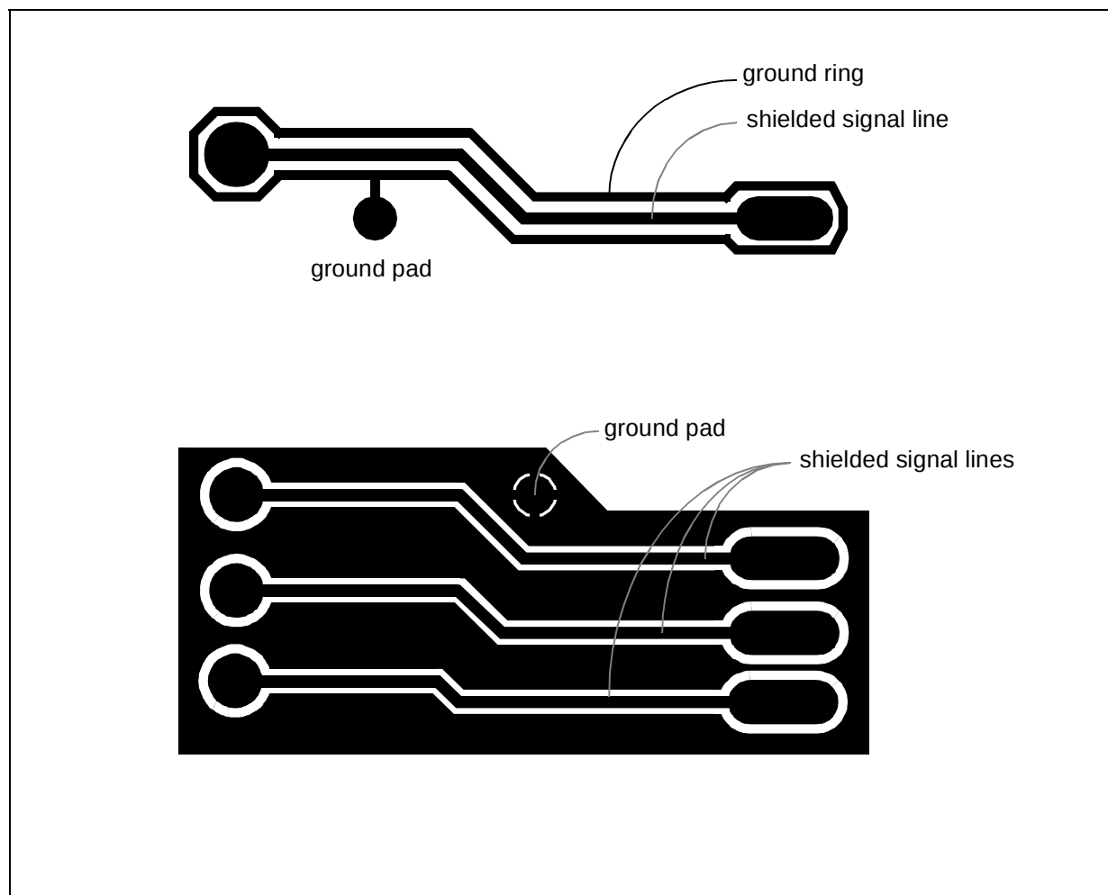
Figure 6-7. Shielding signals
