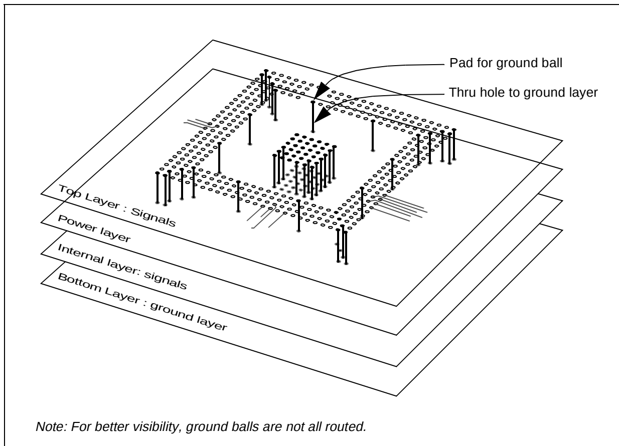
Figure 6-8. Ground routing
