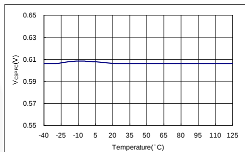
Figure 14. PFC Peak Current Limit Voltage
