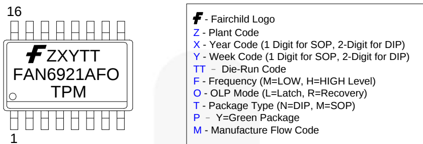
Figure 3. Marking Diagram
