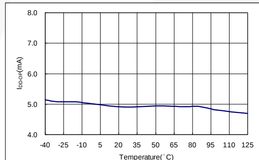
Figure 10. Operating Current
