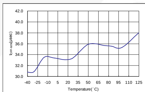
Figure 20. PWM Minimum Off Time for V_{FB}=V_G
