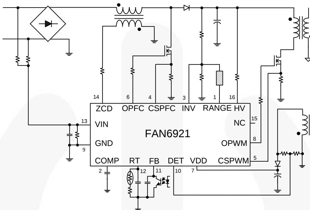
Figure 1. Typical Application
