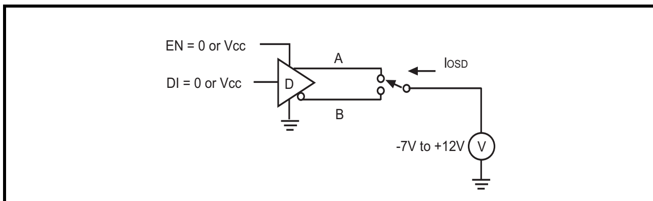
FIGURE 5. RS-485 DRIVER PROPAGATION DELAY TEST CIRCUIT
