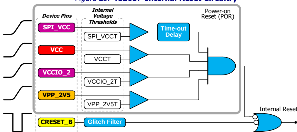
Figure 25: iCE65P Internal Reset Circuitry
