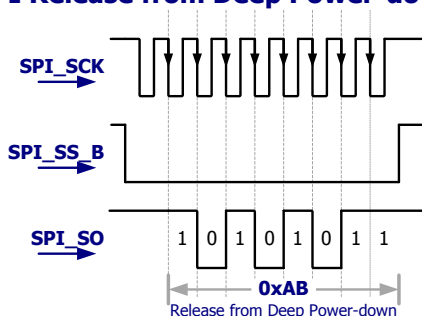
Figure 27: SPI Release from Deep Power-down Command
