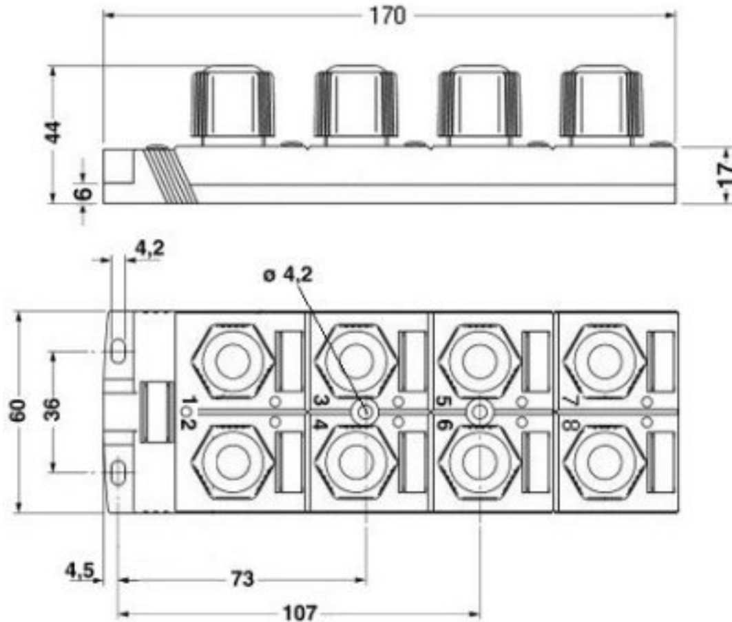
Dimensioned drawing
