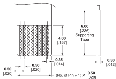
Recommended FPC Layout
