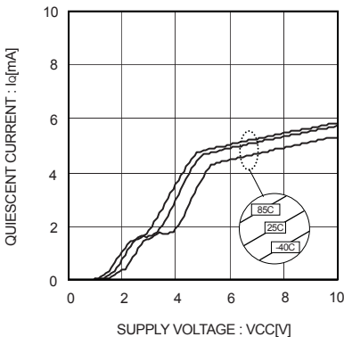
Fig.4 Quiescent current vs Supply voltage (BD3824FS)
