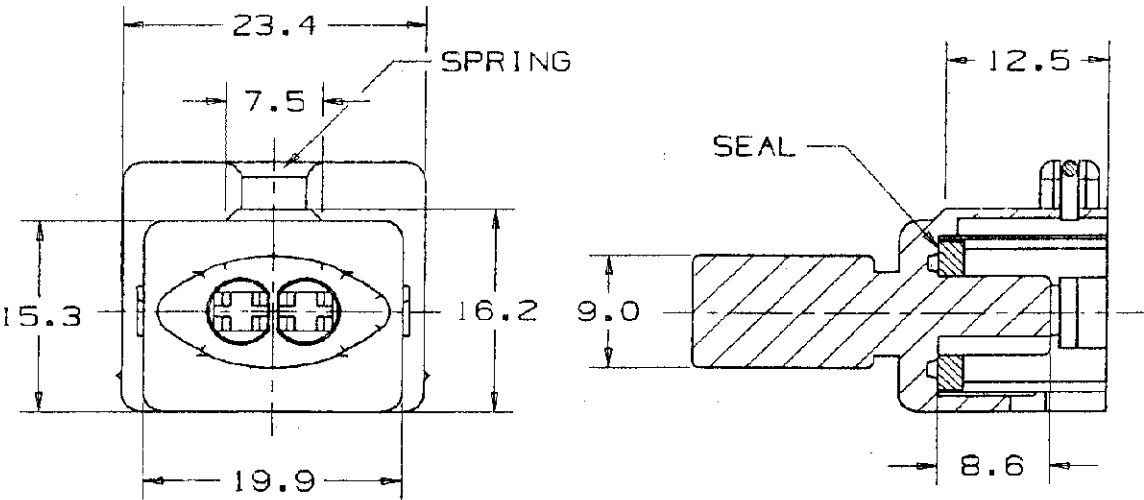
SECTION X-X
