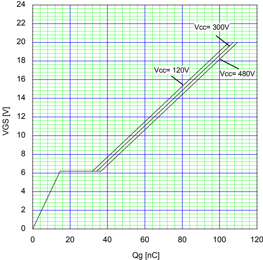
Typical Gate Charge Characteristics V_{GS}=f(Q_g):I_D=17A,T_{ch}=25^{\circ}C
