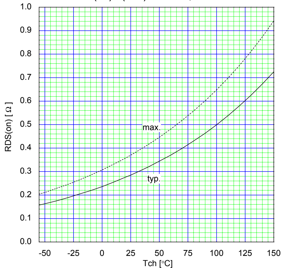
Drain-Source On-state Resistance R_{DS(on)}=f(T_{ch}) : I_D=8.5\text{A} , V_{GS}=10\text{V}
