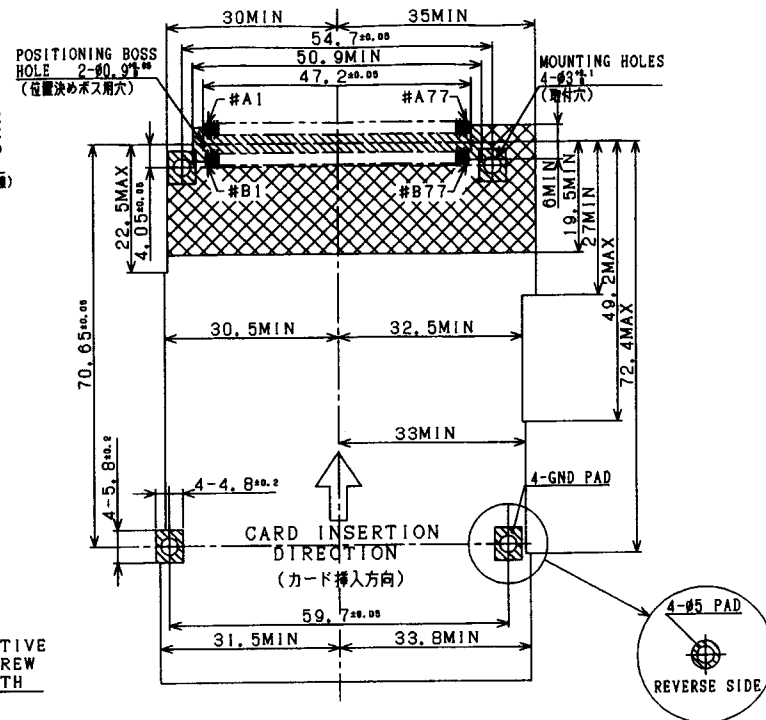
RECOMMENDED P. C. BOARD LAYOUT (MOUNTING FACE SIDE)
