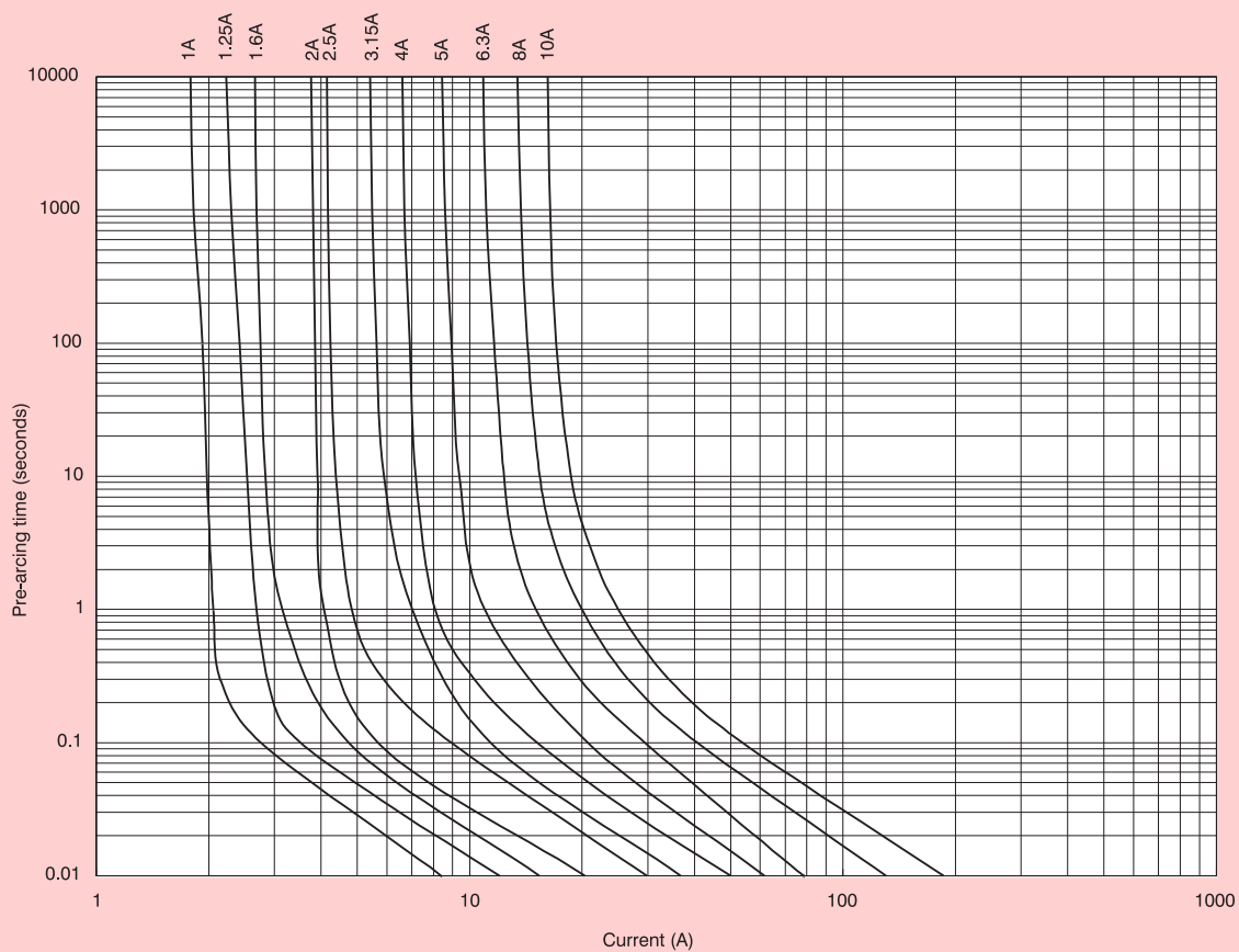
S500, GDB and GDB-V Range: 1A to 10A
