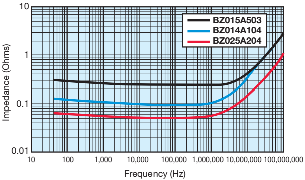
Impedance Comparison
