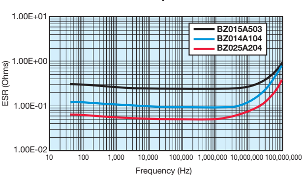
ESR Comparison
