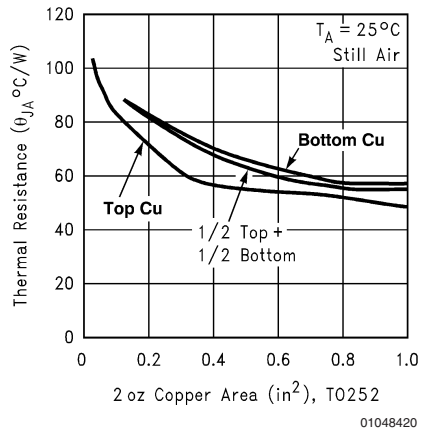
FIGURE 3. \theta_{JA} vs. 2oz Copper Area for TO-252
