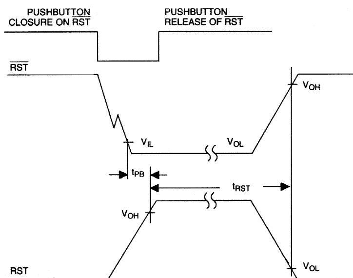
PUSHBUTTON RESET TIMING Figure 4
